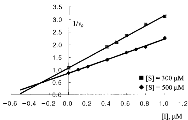
Figure 1. The Dixon plot for the inhibition of CPA with racemic 2-benzyl-2-methylsuccinic acid (substrate, Hipp-L-Phe; Tris buffer of pH 7.5; temperature, 25°C).
