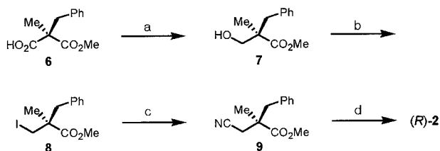
Scheme 2. (a) Isobutyl chloroformate (1 equiv), NMM (1 equiv), DME, -15^\circ\text{C} , 15 min; \text{NaBH}_4 (3 equiv), -15^\circ\text{C} , 10 min, 65%; (b) \text{PPh}_3 (1.2 equiv), \text{I}_2 (1.2 equiv), imidazole (1.2 equiv), toluene, 80^\circ\text{C} , 18 h, 90%; (c) KCN, 18-crown-6, DMSO, 80^\circ\text{C} , 10 h, 90%; (d) 20% NaOH, 90^\circ\text{C} , 24 h, 90%.
