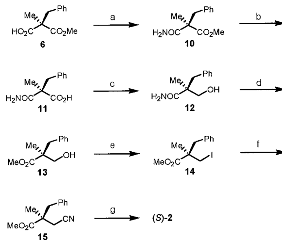
Scheme 3. (a) Isobutyl chloroformate (1 equiv), NMM (1 equiv), DME, -15^\circ\text{C} , 15 min; \text{NH}_4\text{OH} (5 equiv), -15^\circ\text{C} to rt, 2 h, 64%; (b) LiOH, THF/MeOH/ \text{H}_2\text{O} , rt, 12 h, 95%; (c) isobutyl chloroformate (1 equiv), NMM (1 equiv), DME, -15^\circ\text{C} ; \text{NaBH}_4 (3 equiv), -15^\circ\text{C} to rt, 1 h, 70%; (d) MeOH, HCl, reflux, 24 h, 80%; (e) \text{PPh}_3 (1.2 equiv), \text{I}_2 (1.2 equiv), imidazole (1.2 equiv), toluene, 80^\circ\text{C} , 18 h, 89%; (f) KCN, 18-crown-6, DMSO, 80^\circ\text{C} , 10 h, 90%; (g) 20% NaOH, 90^\circ\text{C} , 24 h, 90%.
