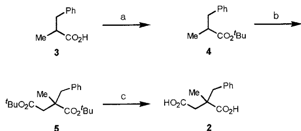
Scheme 1. (a) Isobutylene, \text{H}_2\text{SO}_4 , \text{CH}_2\text{Cl}_2 , rt, 3 d, 90%; (b) LDA (1.2 equiv), THF, 0^\circ\text{C} ; butyl bromoacetate (2.0 equiv), 0^\circ\text{C} to rt, 4 h, 65%; (c) \text{CF}_3\text{CO}_2\text{H} , rt, 1 h, 80%.
